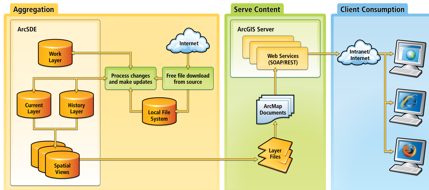
An overview of the aggregated live feed methodology
