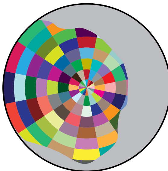
The sky map is further overlaid with the calculated viewshed to calculate the direct solar radiation.
